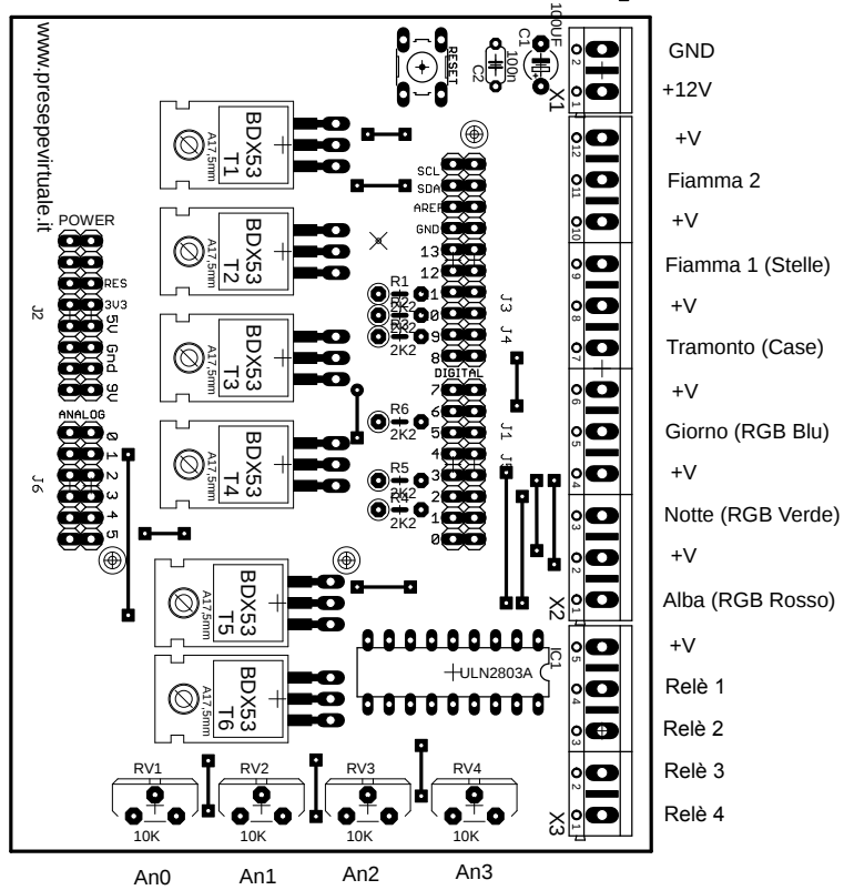
Arduino UNO Shield Centralina 4D+4R+2F LED R.1_1
